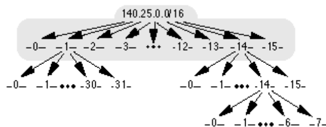
Figure 21: Define the 16 Subnets for 140.25.0.0/16
