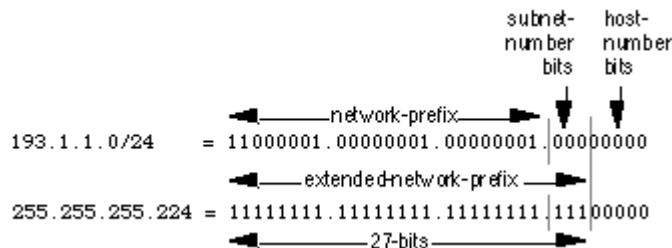
Figure 11: Example #1 - Defining the Subnet Mask/Extended-Prefix Length
