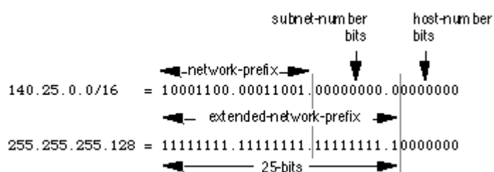
Figure 14: Example #2 - Defining the Subnet Mask/Extended-Prefix Length
