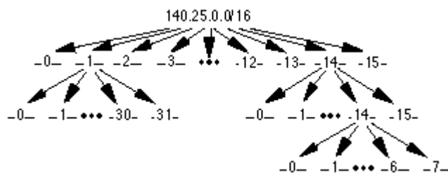
Figure 20: Address Strategy for VLSM Example
