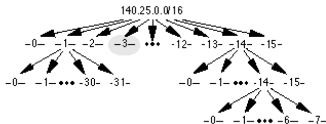
Figure 22: Define the Host Addresses for Subnet #3 (140.25.48.0/20)
