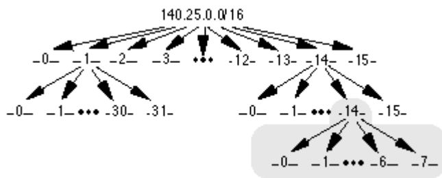
Figure 25: Define the Sub 2 -Subnets for Subnet #14-14 (140.25.238.0/24)
